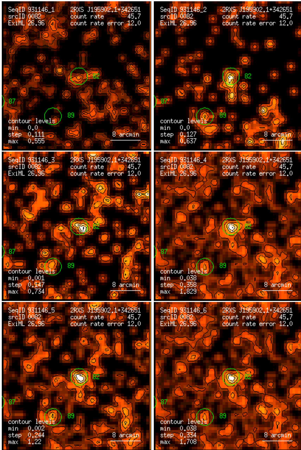
Figure 82: RASS 931146: detection 0082: band rate images, Gaussian filter: (1) PSPC channels 11 – 41, (2) 52 – 90, (3) 91 – 201, (4) 11 – 235, (5) 52 – 201, (6) 11 – 201. Broad band rates in counts/ks. Band rate contour levels in counts/ks/arcmin 2 .
