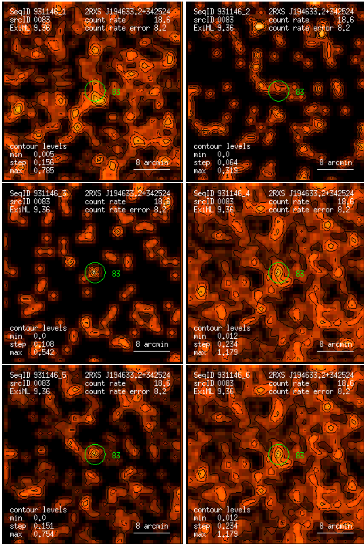
Figure 83: RASS 931146: detection 0083: band rate images, Gaussian filter: (1) PSPC channels 11 – 41, (2) 52 – 90, (3) 91 – 201, (4) 11 – 235, (5) 52 – 201, (6) 11 – 201. Broad band rates in counts/ks. Band rate contour levels in counts/ks/arcmin 2 .
