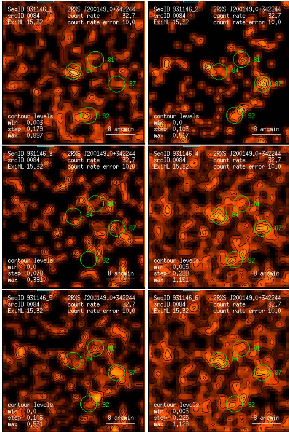
Figure 84: RASS 931146: detection 0084: band rate images, Gaussian filter: (1) PSPC channels 11 – 41, (2) 52 – 90, (3) 91 – 201, (4) 11 – 235, (5) 52 – 201, (6) 11 – 201. Broad band rates in counts/ks. Band rate contour levels in counts/ks/arcmin 2 .
