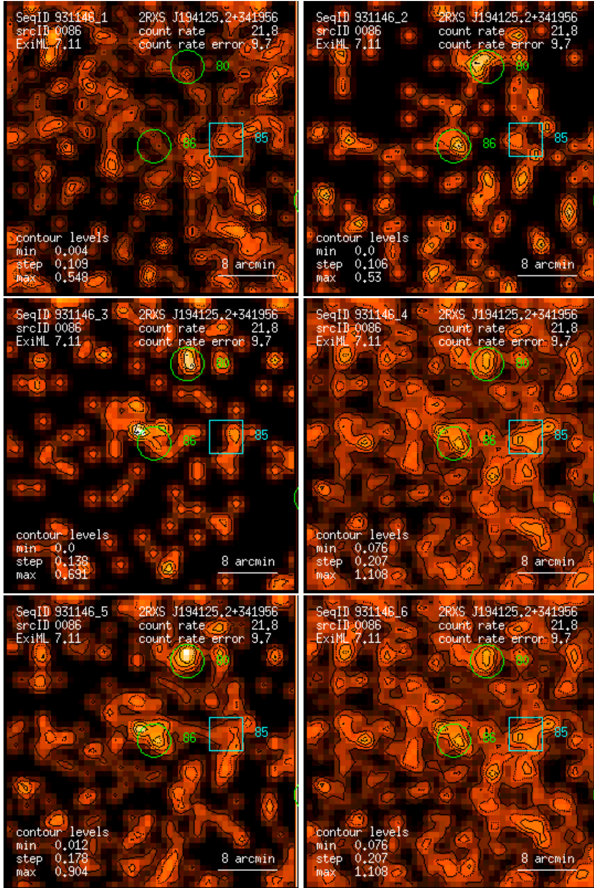
Figure 86: RASS 931146: detection 0086: band rate images, Gaussian filter: (1) PSPC channels 11 – 41, (2) 52 – 90, (3) 91 – 201, (4) 11 – 235, (5) 52 – 201, (6) 11 – 201. Broad band rates in counts/ks. Band rate contour levels in counts/ks/arcmin 2 .
