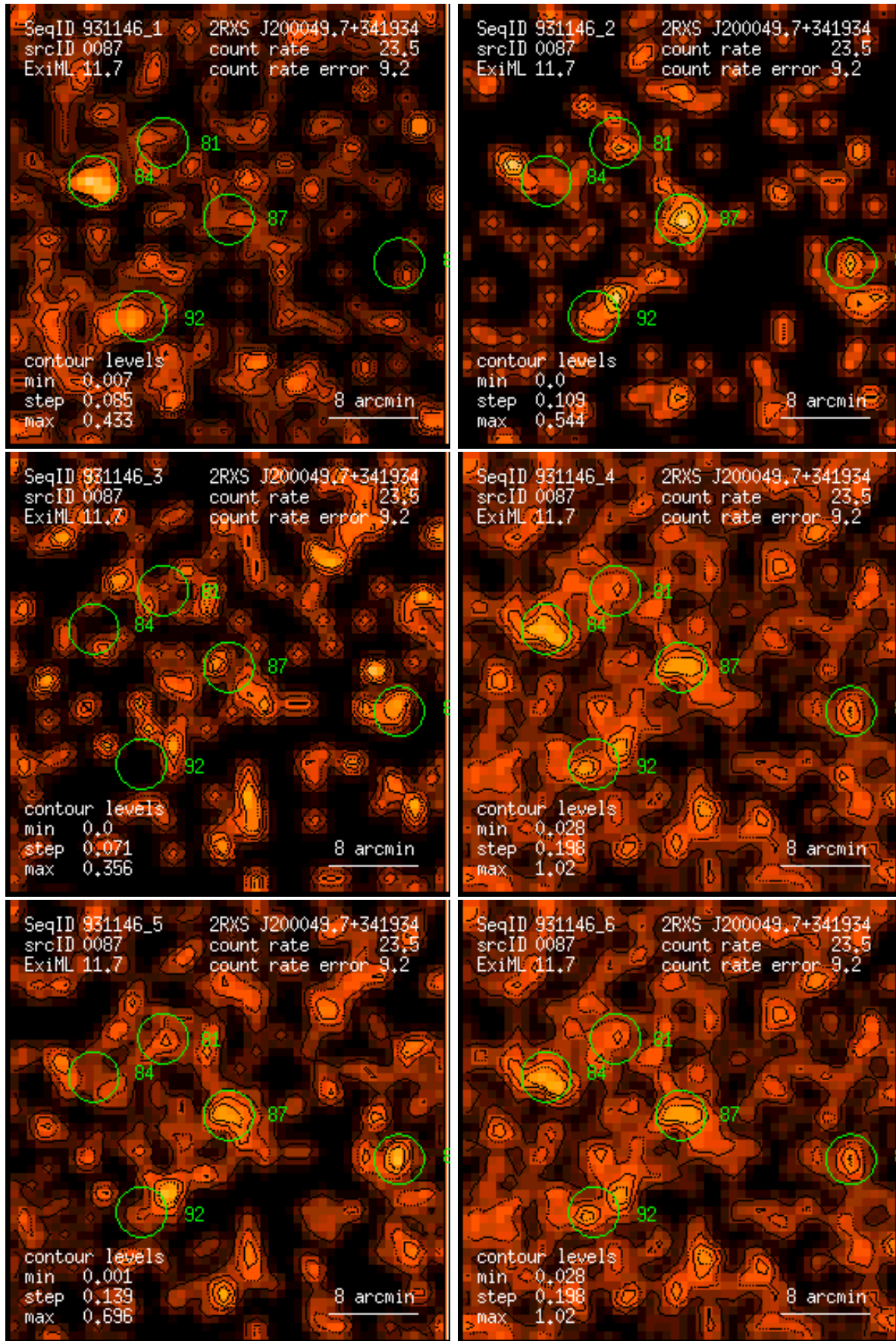
Figure 87: RASS 931146: detection 0087: band rate images, Gaussian filter: (1) PSPC channels 11 – 41, (2) 52 – 90, (3) 91 – 201, (4) 11 – 235, (5) 52 – 201, (6) 11 – 201. Broad band rates in counts/ks. Band rate contour levels in counts/ks/arcmin 2 .
