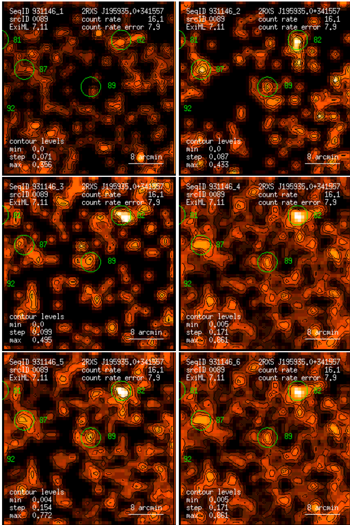
Figure 89: RASS 931146: detection 0089: band rate images, Gaussian filter: (1) PSPC channels 11 – 41, (2) 52 – 90, (3) 91 – 201, (4) 11 – 235, (5) 52 – 201, (6) 11 – 201. Broad band rates in counts/ks. Band rate contour levels in counts/ks/arcmin 2 .
