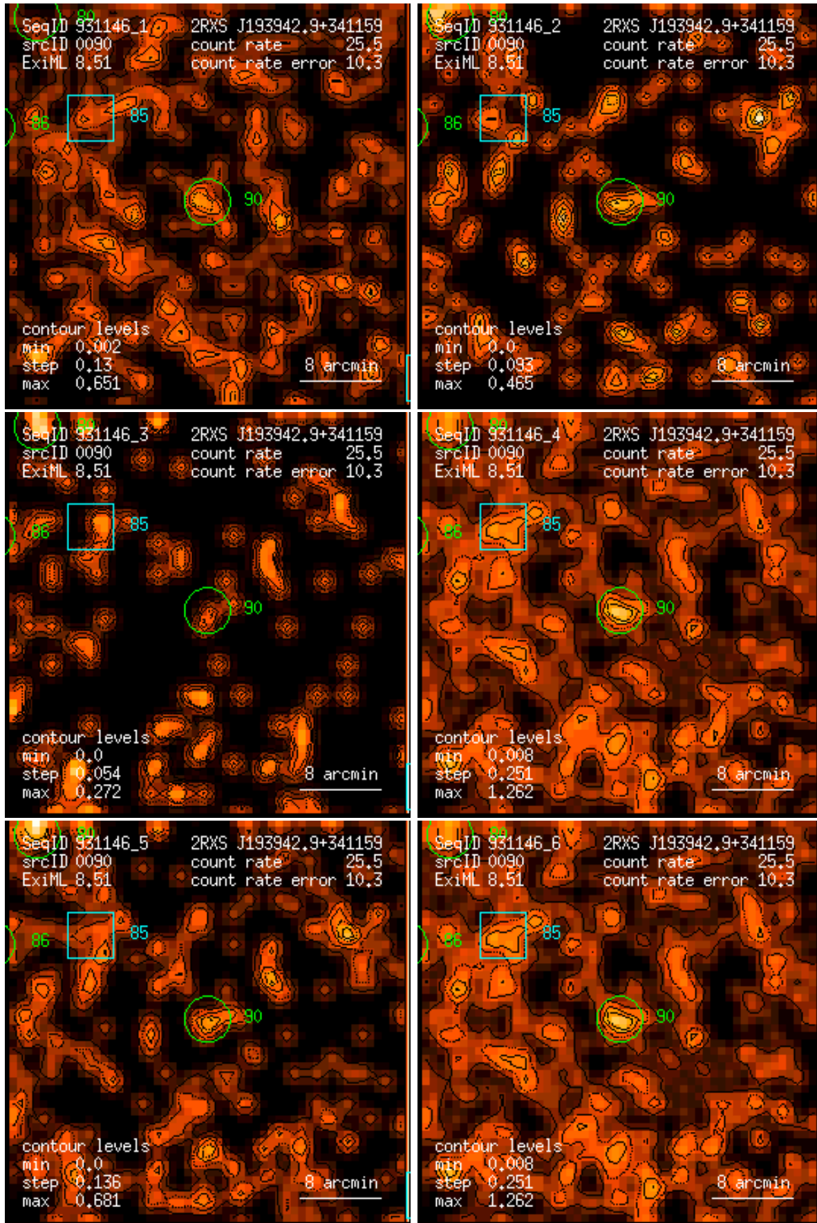
Figure 90: RASS 931146: detection 0090: band rate images, Gaussian filter: (1) PSPC channels 11 – 41, (2) 52 – 90, (3) 91 – 201, (4) 11 – 235, (5) 52 – 201, (6) 11 – 201. Broad band rates in counts/ks. Band rate contour levels in counts/ks/arcmin 2 .
