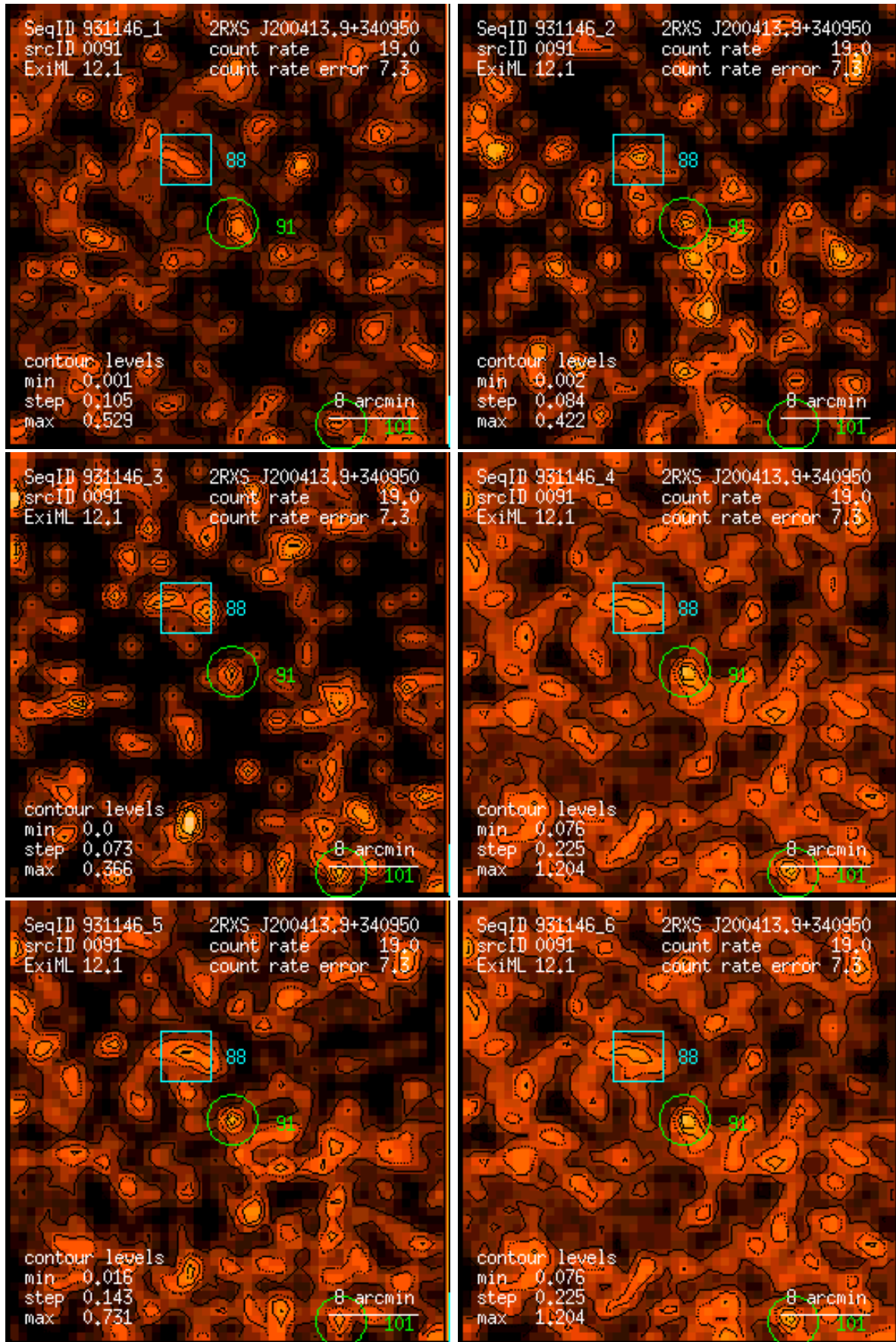
Figure 91: RASS 931146: detection 0091: band rate images, Gaussian filter: (1) PSPC channels 11 – 41, (2) 52 – 90, (3) 91 – 201, (4) 11 – 235, (5) 52 – 201, (6) 11 – 201. Broad band rates in counts/ks. Band rate contour levels in counts/ks/arcmin 2 .
