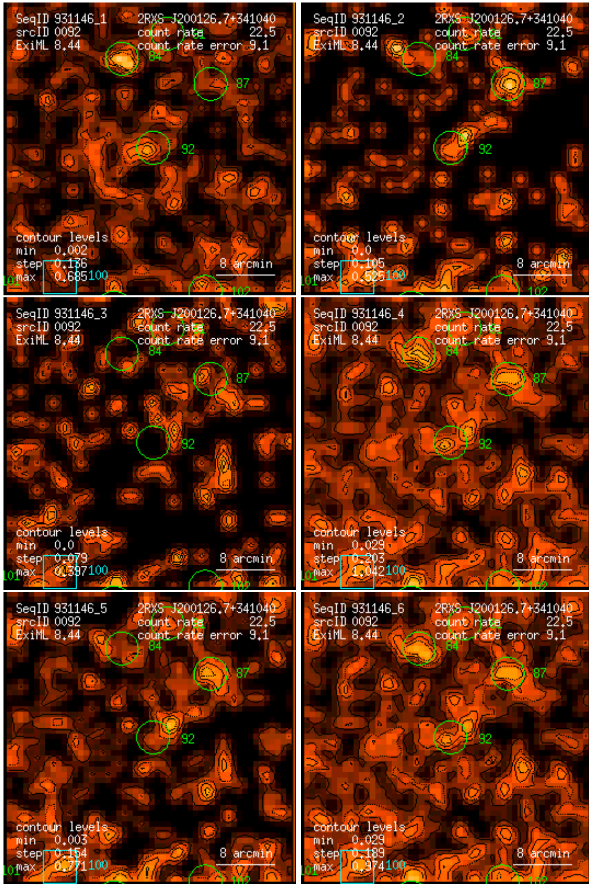
Figure 92: RASS 931146: detection 0092: band rate images, Gaussian filter: (1) PSPC channels 11 – 41, (2) 52 – 90, (3) 91 – 201, (4) 11 – 235, (5) 52 – 201, (6) 11 – 201. Broad band rates in counts/ks. Band rate contour levels in counts/ks/arcmin 2 .
