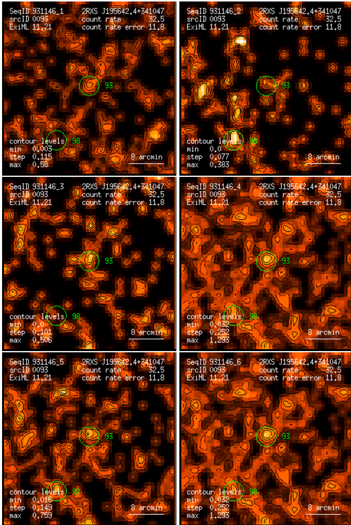
Figure 93: RASS 931146: detection 0093: band rate images, Gaussian filter: (1) PSPC channels 11 – 41, (2) 52 – 90, (3) 91 – 201, (4) 11 – 235, (5) 52 – 201, (6) 11 – 201. Broad band rates in counts/ks. Band rate contour levels in counts/ks/arcmin 2 .
