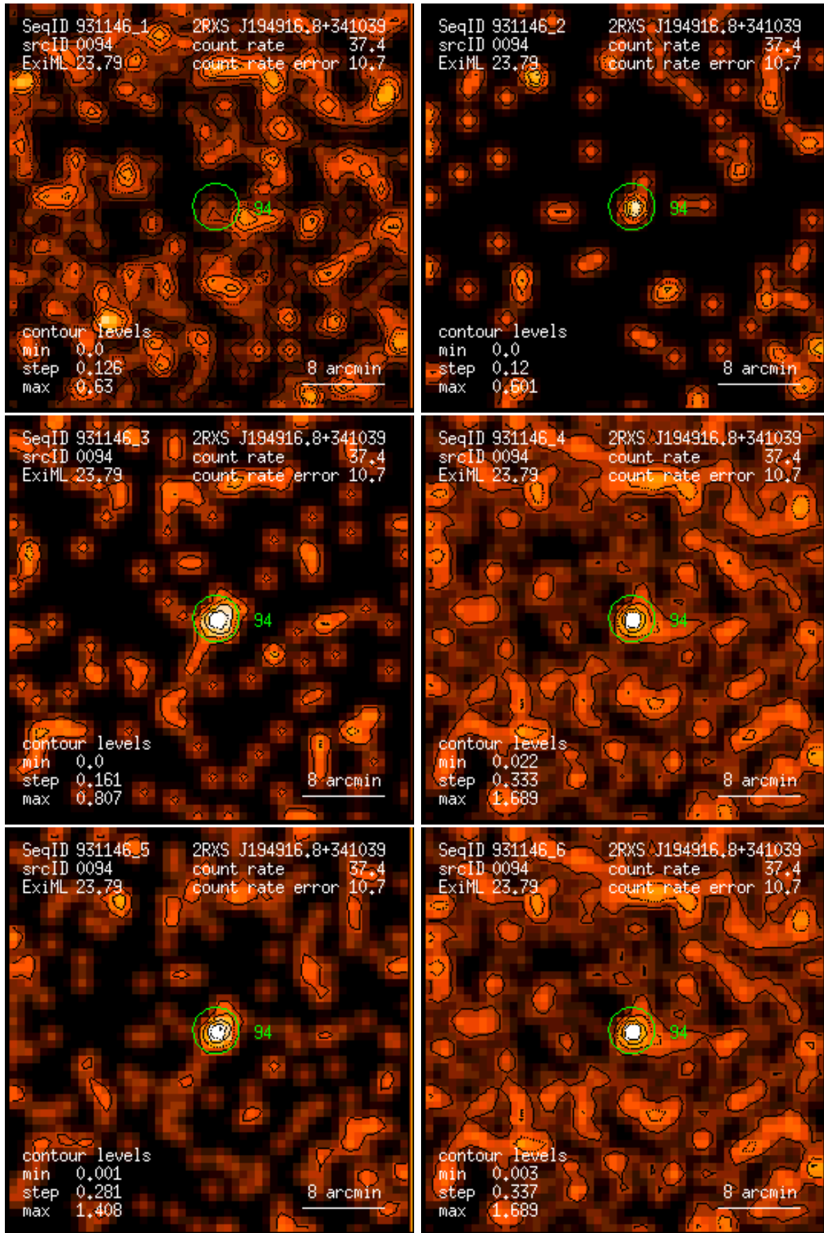
Figure 94: RASS 931146: detection 0094: band rate images, Gaussian filter: (1) PSPC channels 11 – 41, (2) 52 – 90, (3) 91 – 201, (4) 11 – 235, (5) 52 – 201, (6) 11 – 201. Broad band rates in counts/ks. Band rate contour levels in counts/ks/arcmin 2 .
