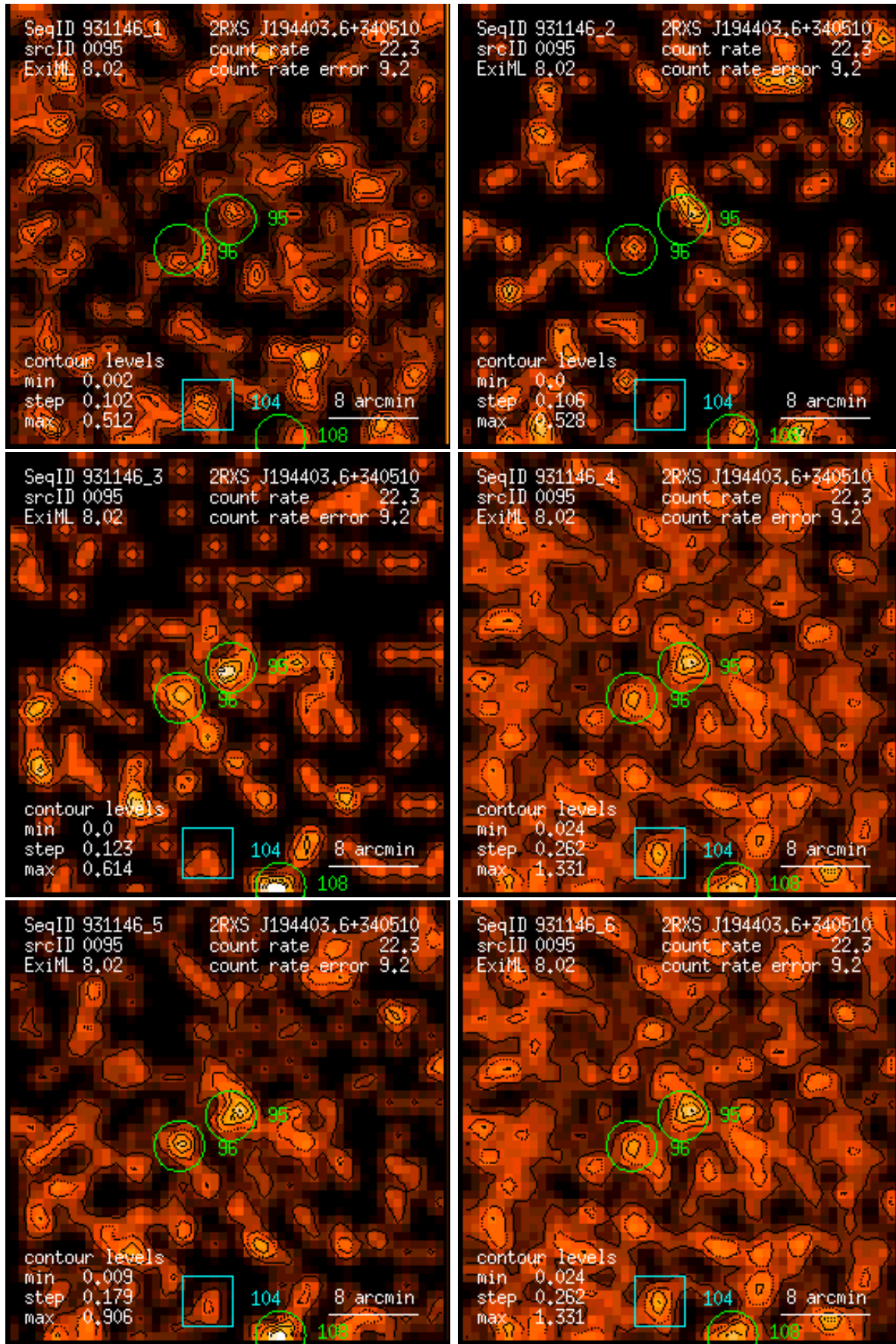
Figure 95: RASS 931146: detection 0095: band rate images, Gaussian filter: (1) PSPC channels 11 – 41, (2) 52 – 90, (3) 91 – 201, (4) 11 – 235, (5) 52 – 201, (6) 11 – 201. Broad band rates in counts/ks. Band rate contour levels in counts/ks/arcmin 2 .
