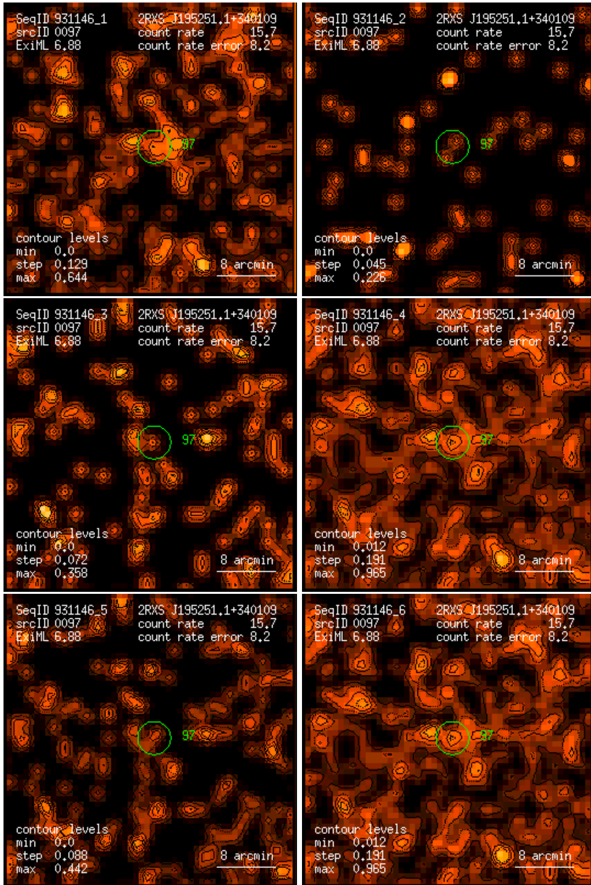
Figure 97: RASS 931146: detection 0097: band rate images, Gaussian filter: (1) PSPC channels 11 – 41, (2) 52 – 90, (3) 91 – 201, (4) 11 – 235, (5) 52 – 201, (6) 11 – 201. Broad band rates in counts/ks. Band rate contour levels in counts/ks/arcmin 2 .
