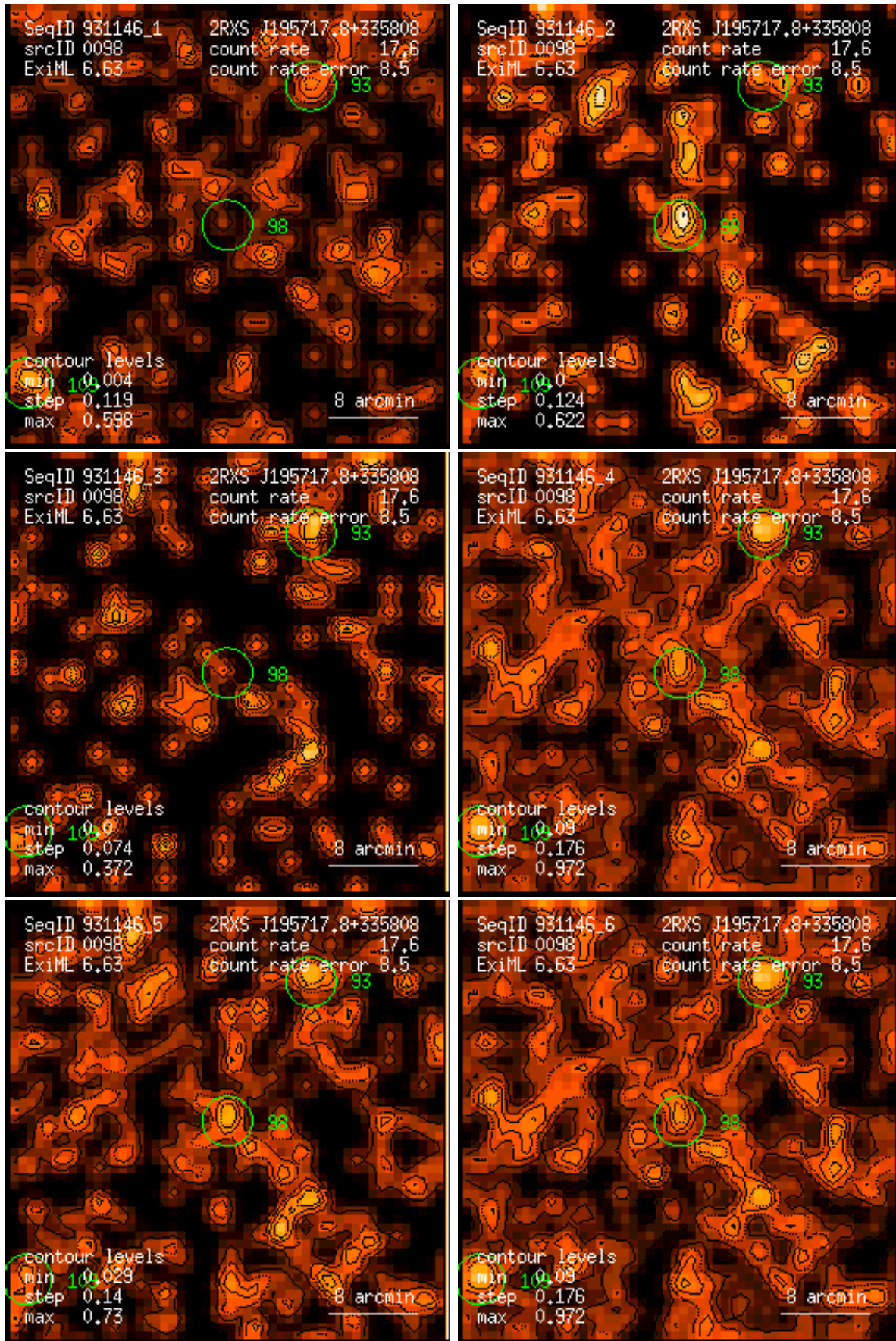
Figure 98: RASS 931146: detection 0098: band rate images, Gaussian filter: (1) PSPC channels 11 – 41, (2) 52 – 90, (3) 91 – 201, (4) 11 – 235, (5) 52 – 201, (6) 11 – 201. Broad band rates in counts/ks. Band rate contour levels in counts/ks/arcmin 2 .
