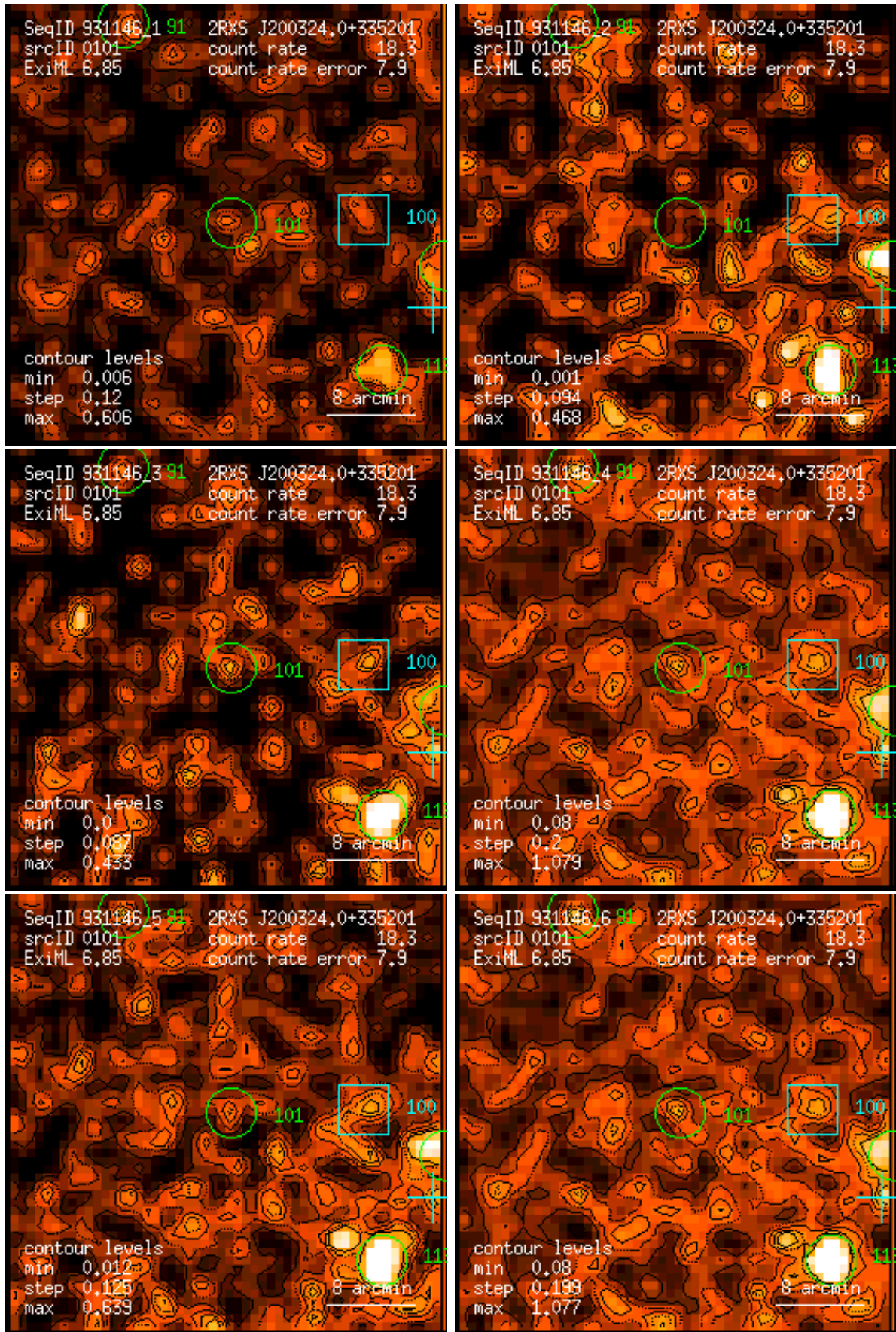
Figure 101: RASS 931146: detection 0101: band rate images, Gaussian filter: (1) PSPC channels 11 – 41, (2) 52 – 90, (3) 91 – 201, (4) 11 – 235, (5) 52 – 201, (6) 11 – 201. Broad band rates in counts/ks. Band rate contour levels in counts/ks/arcmin 2 .
