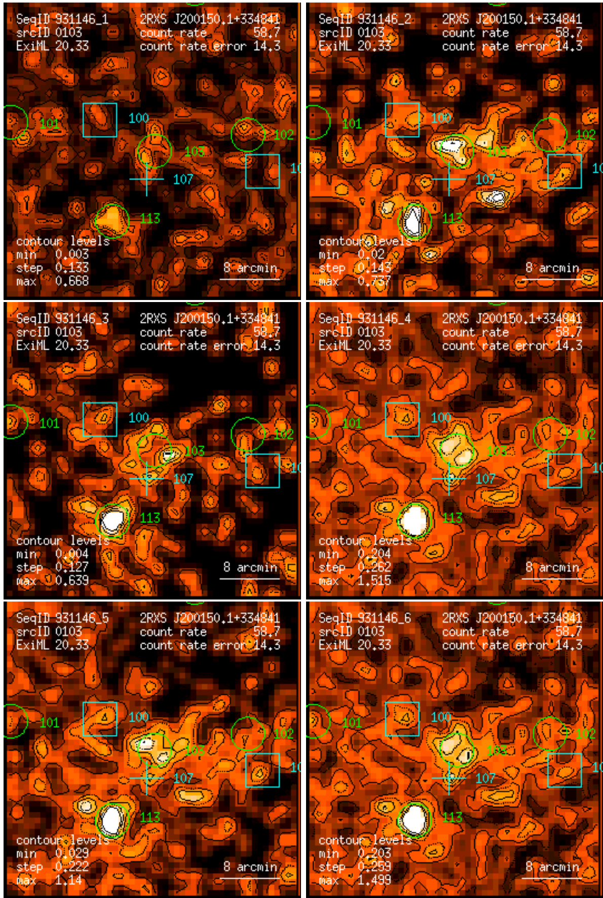
Figure 103: RASS 931146: detection 0103: band rate images, Gaussian filter: (1) PSPC channels 11 – 41, (2) 52 – 90, (3) 91 – 201, (4) 11 – 235, (5) 52 – 201, (6) 11 – 201. Broad band rates in counts/ks. Band rate contour levels in counts/ks/arcmin 2 .
