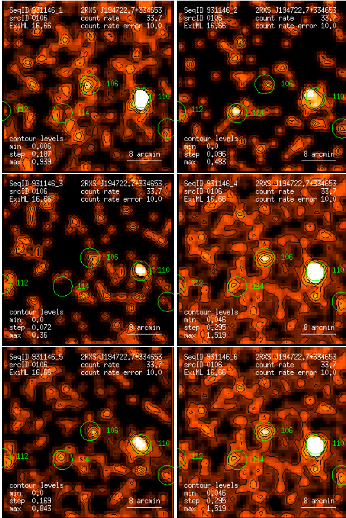
Figure 106: RASS 931146: detection 0106: band rate images, Gaussian filter: (1) PSPC channels 11 – 41, (2) 52 – 90, (3) 91 – 201, (4) 11 – 235, (5) 52 – 201, (6) 11 – 201. Broad band rates in counts/ks. Band rate contour levels in counts/ks/arcmin 2 .
