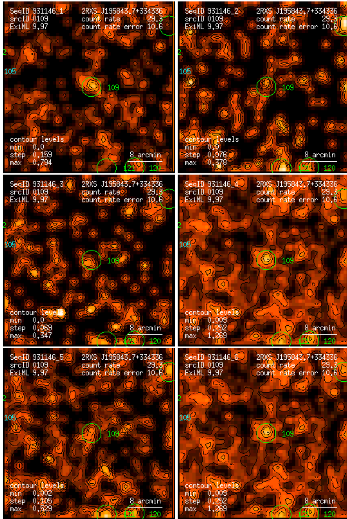
Figure 109: RASS 931146: detection 0109: band rate images, Gaussian filter: (1) PSPC channels 11 – 41, (2) 52 – 90, (3) 91 – 201, (4) 11 – 235, (5) 52 – 201, (6) 11 – 201. Broad band rates in counts/ks. Band rate contour levels in counts/ks/arcmin 2 .
