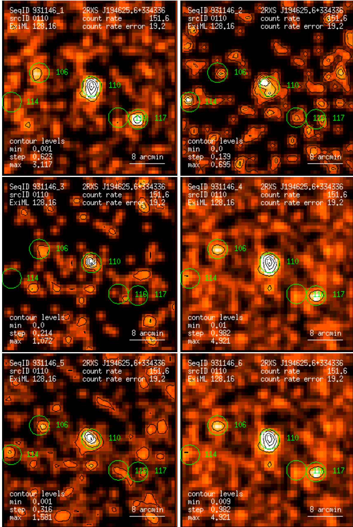
Figure 110: RASS 931146: detection 0110: band rate images, Gaussian filter: (1) PSPC channels 11 – 41, (2) 52 – 90, (3) 91 – 201, (4) 11 – 235, (5) 52 – 201, (6) 11 – 201. Broad band rates in counts/ks. Band rate contour levels in counts/ks/arcmin 2 .
