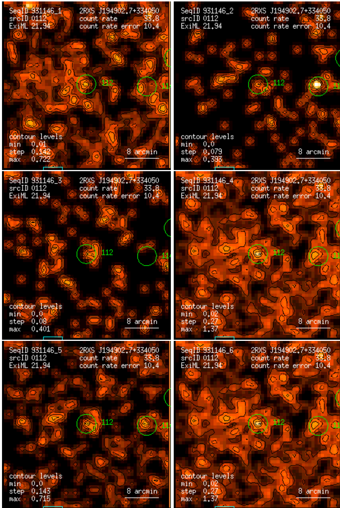
Figure 112: RASS 931146: detection 0112: band rate images, Gaussian filter: (1) PSPC channels 11 – 41, (2) 52 – 90, (3) 91 – 201, (4) 11 – 235, (5) 52 – 201, (6) 11 – 201. Broad band rates in counts/ks. Band rate contour levels in counts/ks/arcmin 2 .
