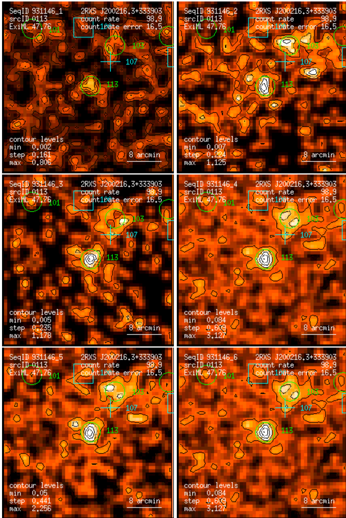
Figure 113: RASS 931146: detection 0113: band rate images, Gaussian filter: (1) PSPC channels 11 – 41, (2) 52 – 90, (3) 91 – 201, (4) 11 – 235, (5) 52 – 201, (6) 11 – 201. Broad band rates in counts/ks. Band rate contour levels in counts/ks/arcmin 2 .
