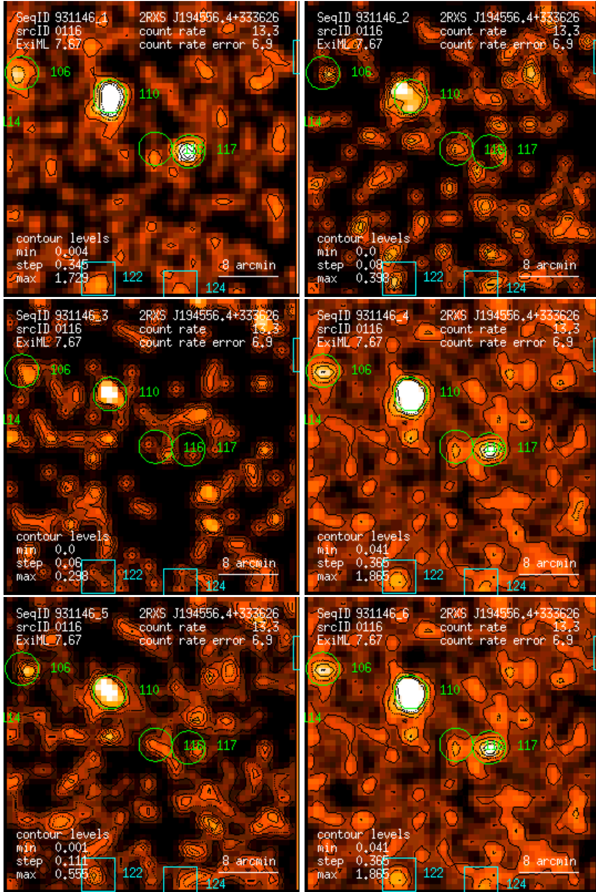
Figure 116: RASS 931146: detection 0116: band rate images, Gaussian filter: (1) PSPC channels 11 – 41, (2) 52 – 90, (3) 91 – 201, (4) 11 – 235, (5) 52 – 201, (6) 11 – 201. Broad band rates in counts/ks. Band rate contour levels in counts/ks/arcmin 2 .
