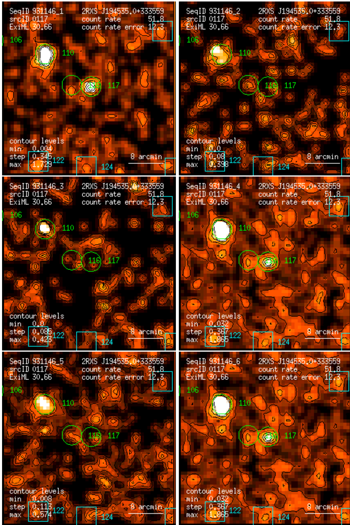
Figure 117: RASS 931146: detection 0117: band rate images, Gaussian filter: (1) PSPC channels 11 – 41, (2) 52 – 90, (3) 91 – 201, (4) 11 – 235, (5) 52 – 201, (6) 11 – 201. Broad band rates in counts/ks. Band rate contour levels in counts/ks/arcmin 2 .
