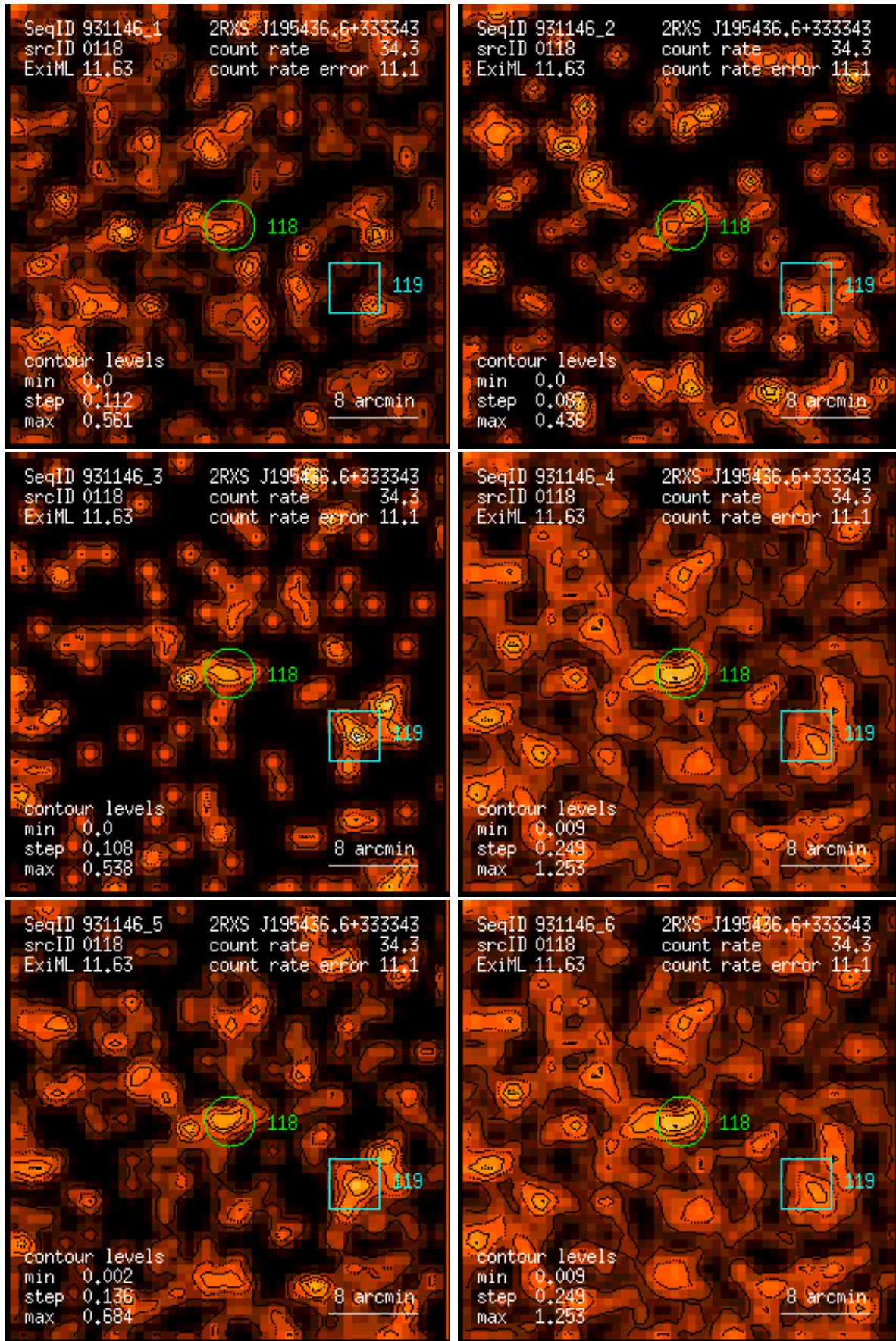
Figure 118: RASS 931146: detection 0118: band rate images, Gaussian filter: (1) PSPC channels 11 – 41, (2) 52 – 90, (3) 91 – 201, (4) 11 – 235, (5) 52 – 201, (6) 11 – 201. Broad band rates in counts/ks. Band rate contour levels in counts/ks/arcmin 2 .
