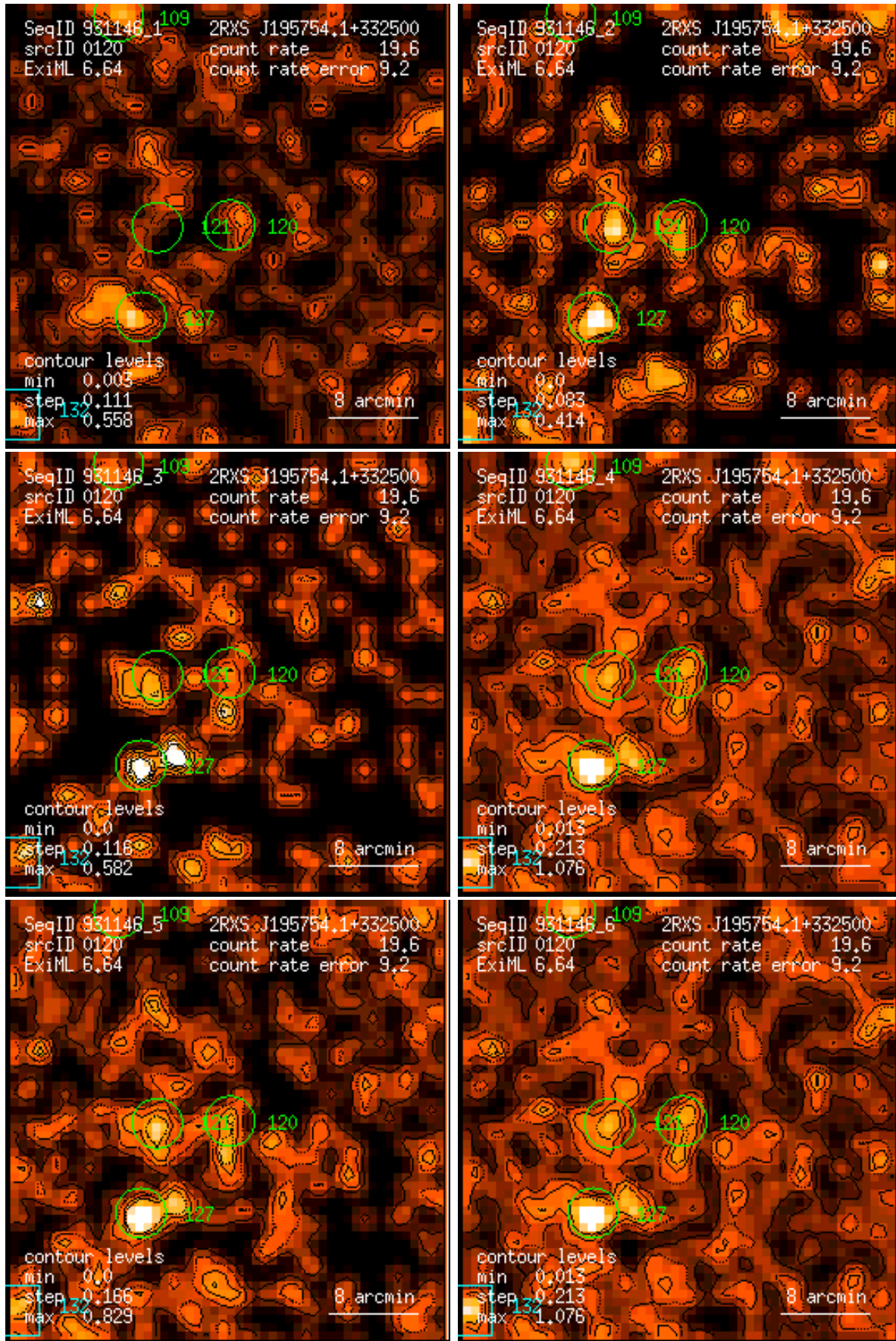
Figure 120: RASS 931146: detection 0120: band rate images, Gaussian filter: (1) PSPC channels 11 – 41, (2) 52 – 90, (3) 91 – 201, (4) 11 – 235, (5) 52 – 201, (6) 11 – 201. Broad band rates in counts/ks. Band rate contour levels in counts/ks/arcmin 2 .
