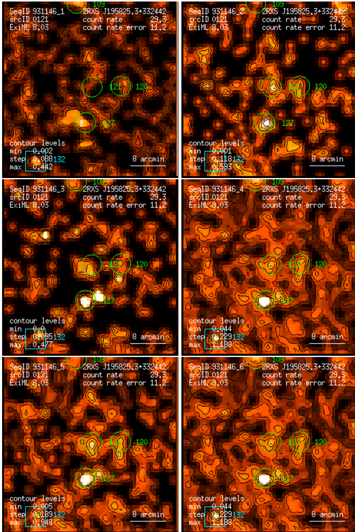
Figure 121: RASS 931146: detection 0121: band rate images, Gaussian filter: (1) PSPC channels 11 – 41, (2) 52 – 90, (3) 91 – 201, (4) 11 – 235, (5) 52 – 201, (6) 11 – 201. Broad band rates in counts/ks. Band rate contour levels in counts/ks/arcmin 2 .
