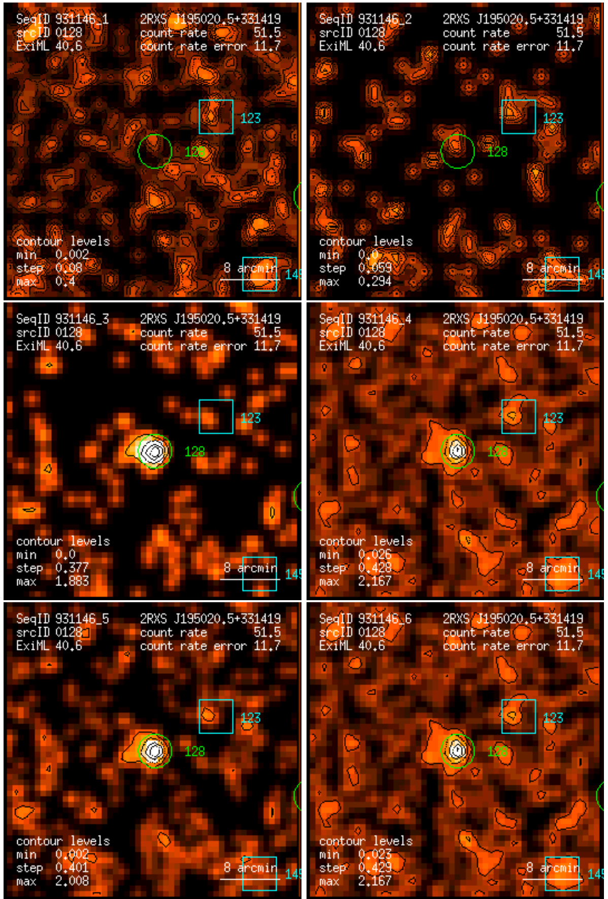
Figure 128: RASS 931146: detection 0128: band rate images, Gaussian filter: (1) PSPC channels 11 – 41, (2) 52 – 90, (3) 91 – 201, (4) 11 – 235, (5) 52 – 201, (6) 11 – 201. Broad band rates in counts/ks. Band rate contour levels in counts/ks/arcmin 2 .
