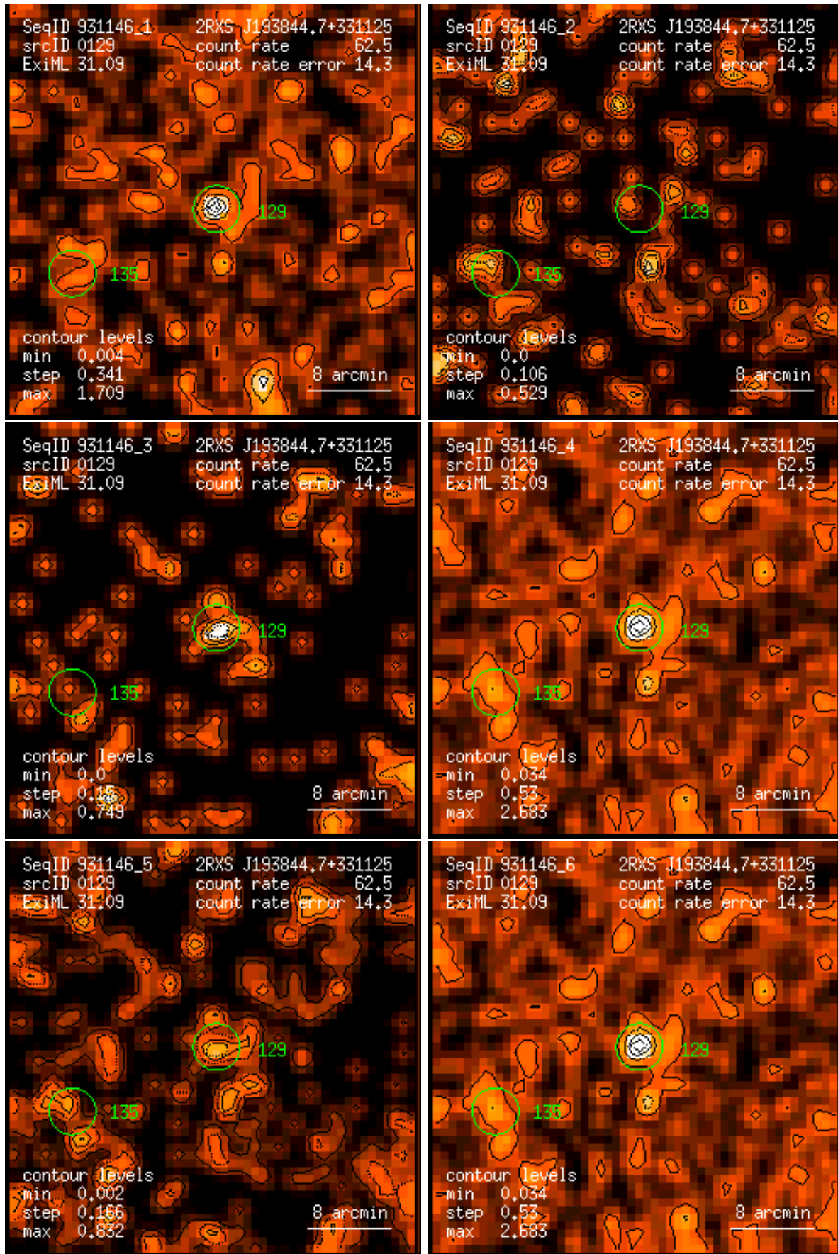
Figure 129: RASS 931146: detection 0129: band rate images, Gaussian filter: (1) PSPC channels 11 – 41, (2) 52 – 90, (3) 91 – 201, (4) 11 – 235, (5) 52 – 201, (6) 11 – 201. Broad band rates in counts/ks. Band rate contour levels in counts/ks/arcmin 2 .
