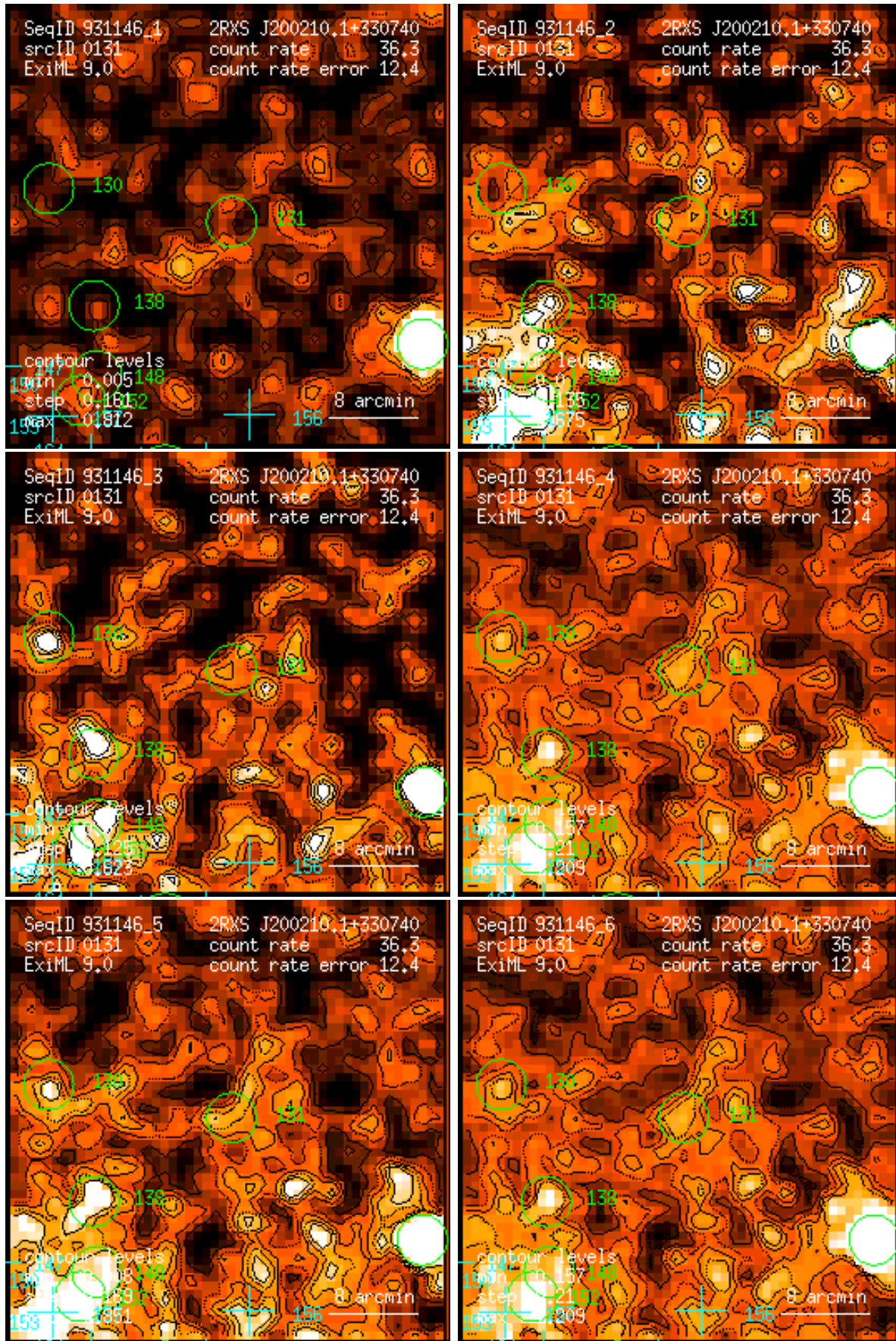
Figure 131: RASS 931146: detection 0131: band rate images, Gaussian filter: (1) PSPC channels 11 – 41, (2) 52 – 90, (3) 91 – 201, (4) 11 – 235, (5) 52 – 201, (6) 11 – 201. Broad band rates in counts/ks. Band rate contour levels in counts/ks/arcmin 2 .
