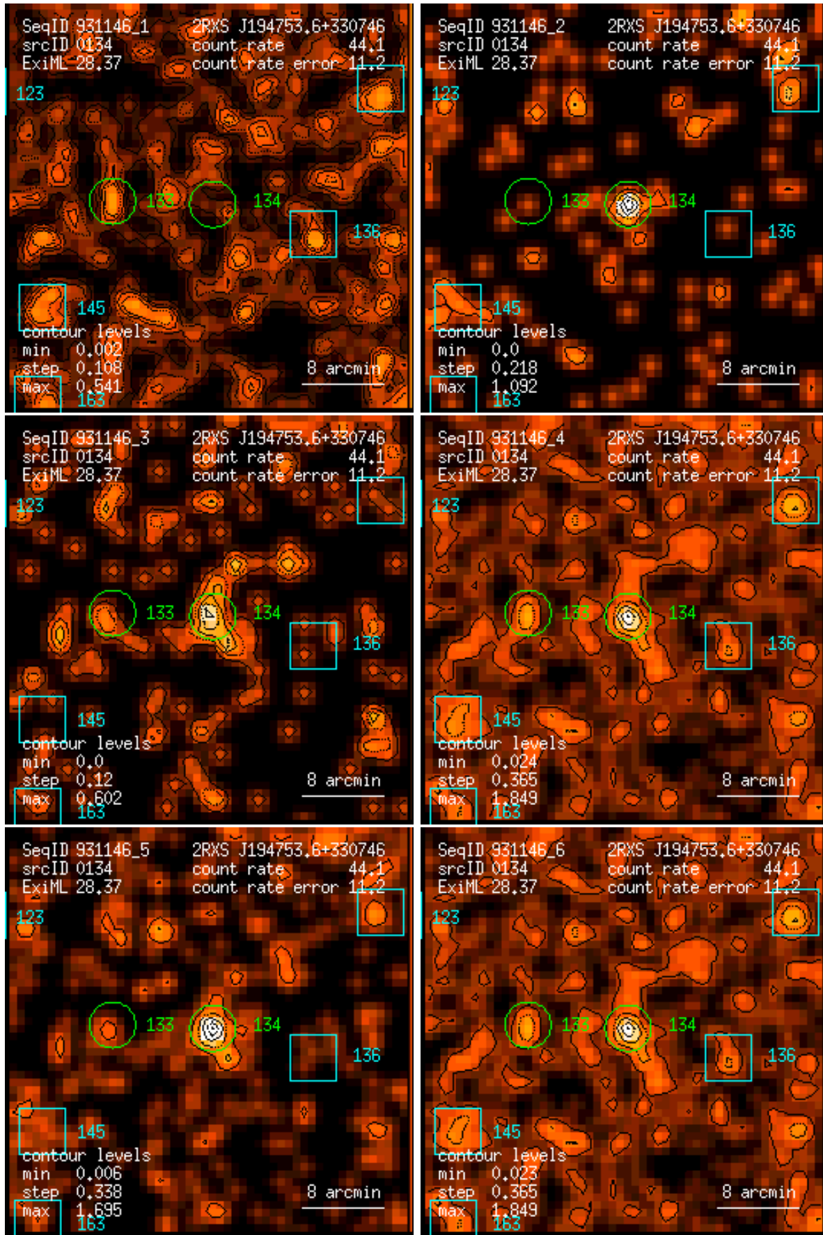
Figure 134: RASS 931146: detection 0134: band rate images, Gaussian filter: (1) PSPC channels 11 – 41, (2) 52 – 90, (3) 91 – 201, (4) 11 – 235, (5) 52 – 201, (6) 11 – 201. Broad band rates in counts/ks. Band rate contour levels in counts/ks/arcmin 2 .
