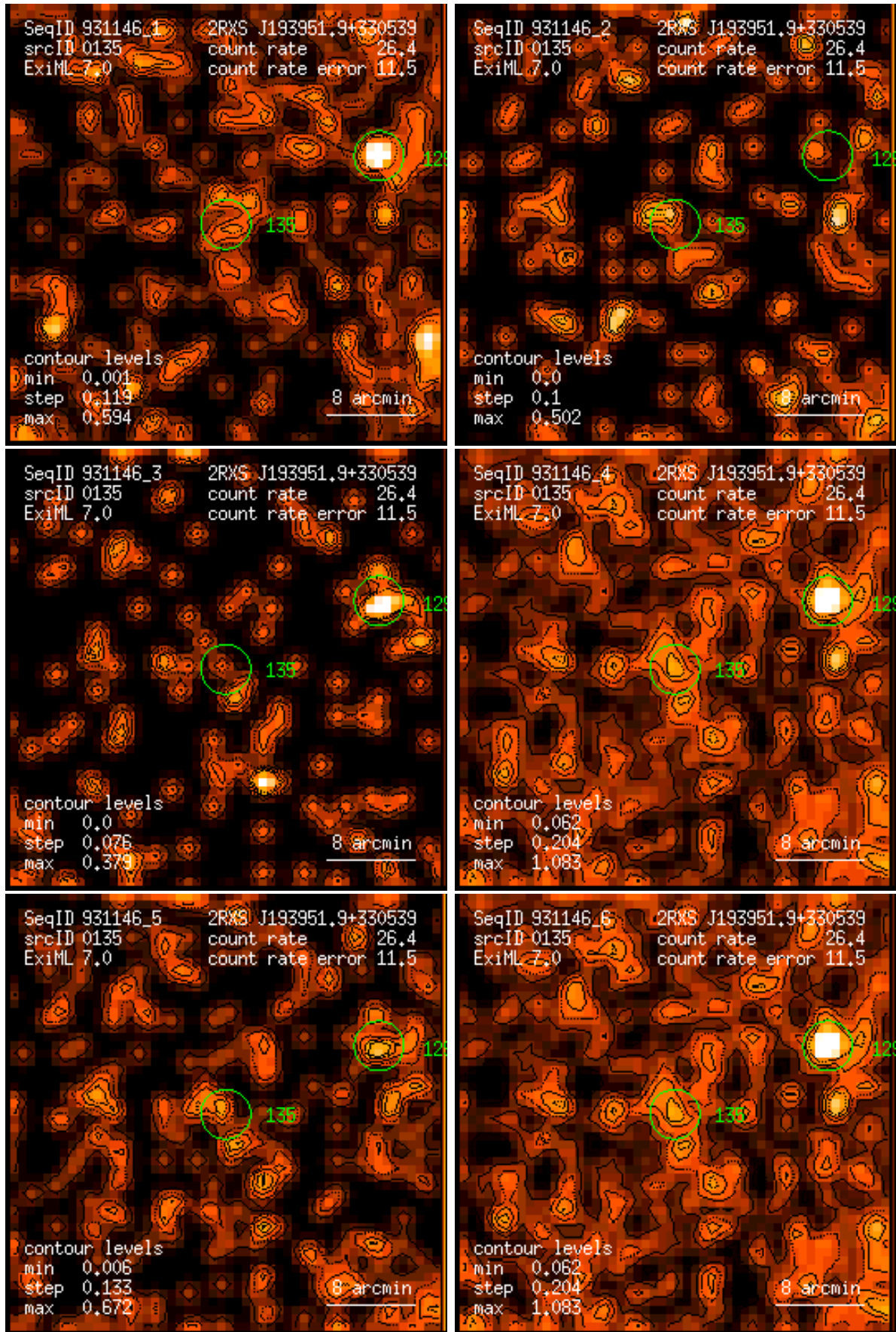
Figure 135: RASS 931146: detection 0135: band rate images, Gaussian filter: (1) PSPC channels 11 – 41, (2) 52 – 90, (3) 91 – 201, (4) 11 – 235, (5) 52 – 201, (6) 11 – 201. Broad band rates in counts/ks. Band rate contour levels in counts/ks/arcmin 2 .
