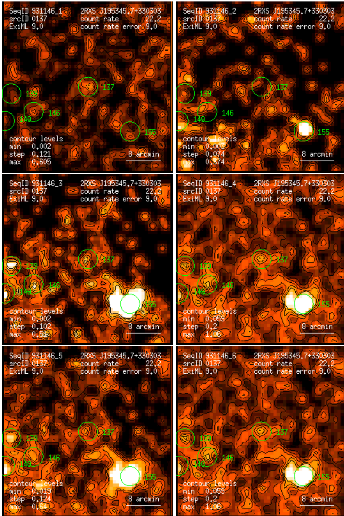
Figure 137: RASS 931146: detection 0137: band rate images, Gaussian filter: (1) PSPC channels 11 – 41, (2) 52 – 90, (3) 91 – 201, (4) 11 – 235, (5) 52 – 201, (6) 11 – 201. Broad band rates in counts/ks. Band rate contour levels in counts/ks/arcmin 2 .
