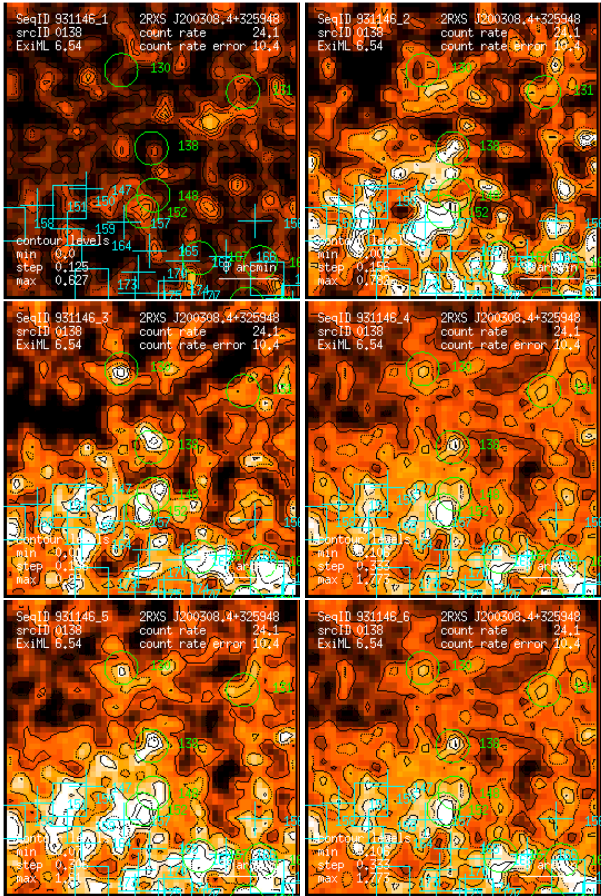
Figure 138: RASS 931146: detection 0138: band rate images, Gaussian filter: (1) PSPC channels 11 – 41, (2) 52 – 90, (3) 91 – 201, (4) 11 – 235, (5) 52 – 201, (6) 11 – 201. Broad band rates in counts/ks. Band rate contour levels in counts/ks/arcmin 2 .
