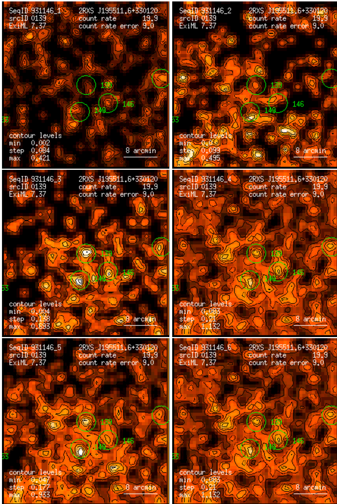
Figure 139: RASS 931146: detection 0139: band rate images, Gaussian filter: (1) PSPC channels 11 – 41, (2) 52 – 90, (3) 91 – 201, (4) 11 – 235, (5) 52 – 201, (6) 11 – 201. Broad band rates in counts/ks. Band rate contour levels in counts/ks/arcmin 2 .
