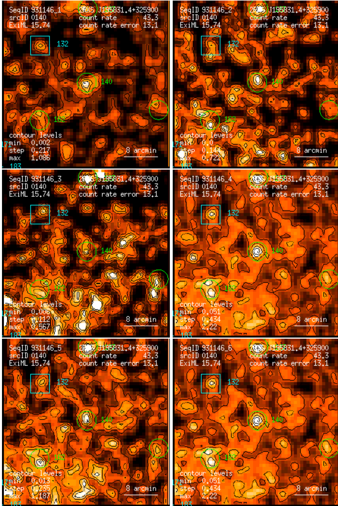
Figure 140: RASS 931146: detection 0140: band rate images, Gaussian filter: (1) PSPC channels 11 – 41, (2) 52 – 90, (3) 91 – 201, (4) 11 – 235, (5) 52 – 201, (6) 11 – 201. Broad band rates in counts/ks. Band rate contour levels in counts/ks/arcmin 2 .
