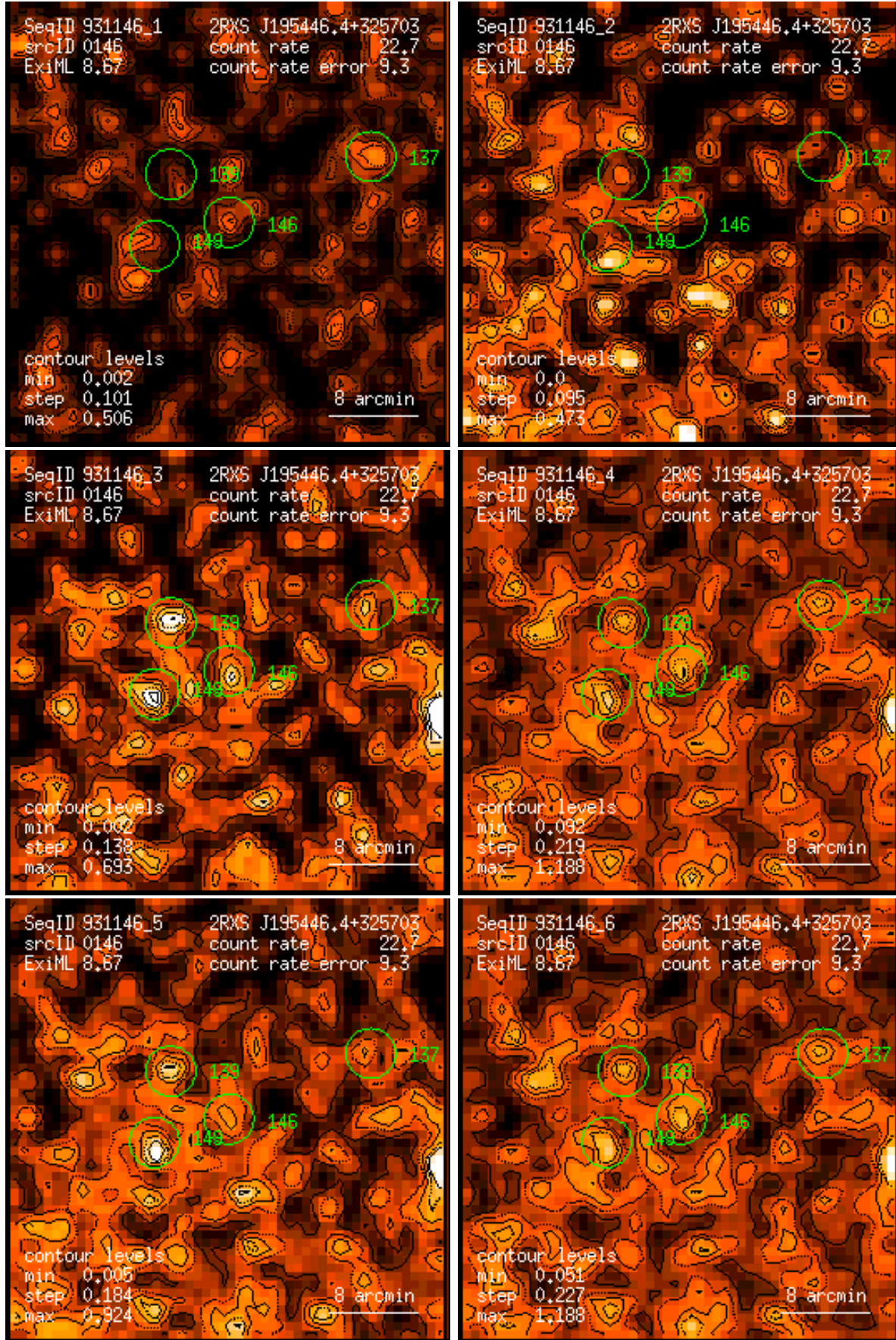
Figure 146: RASS 931146: detection 0146: band rate images, Gaussian filter: (1) PSPC channels 11 – 41, (2) 52 – 90, (3) 91 – 201, (4) 11 – 235, (5) 52 – 201, (6) 11 – 201. Broad band rates in counts/ks. Band rate contour levels in counts/ks/arcmin 2 .
