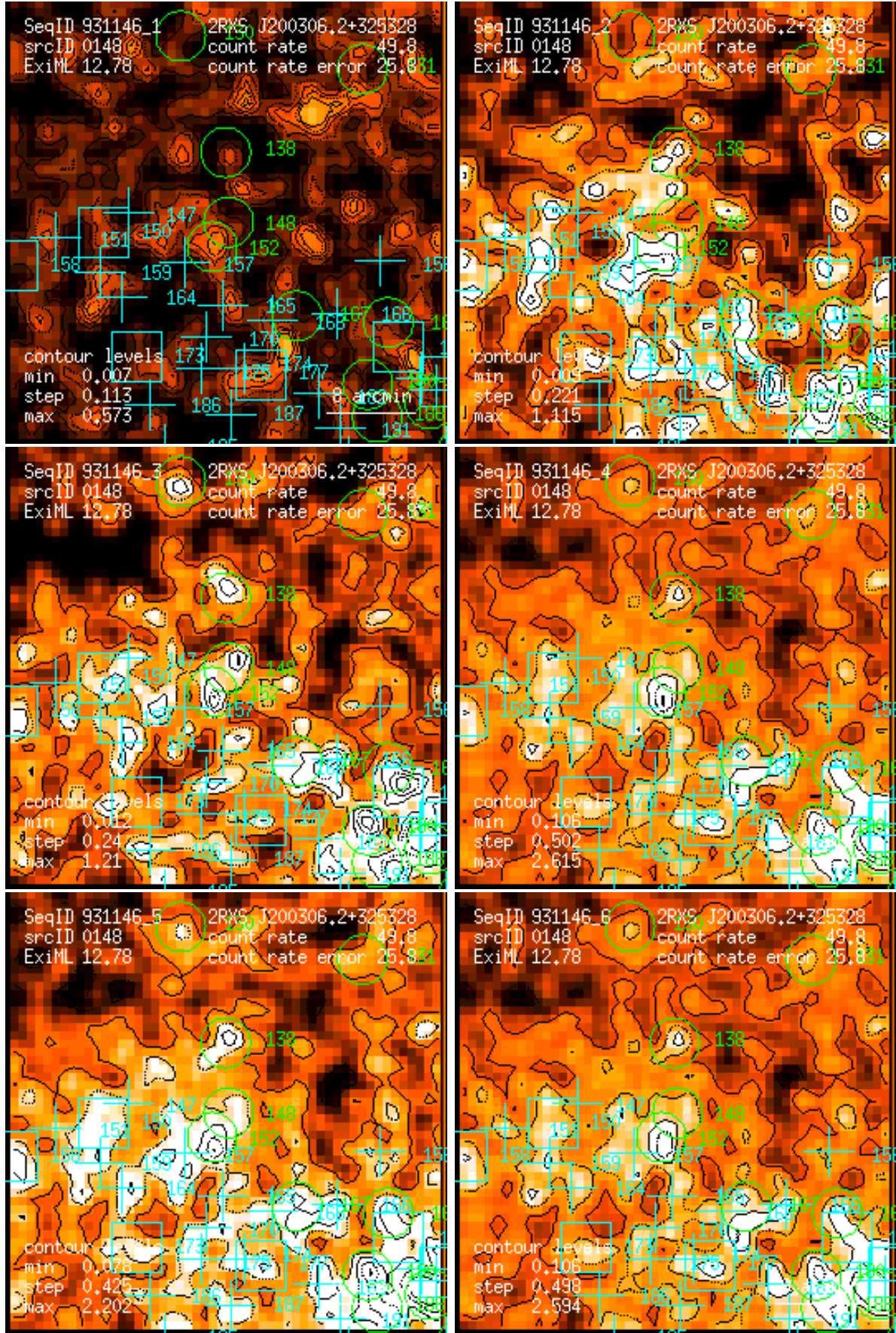
Figure 148: RASS 931146: detection 0148: band rate images, Gaussian filter: (1) PSPC channels 11 – 41, (2) 52 – 90, (3) 91 – 201, (4) 11 – 235, (5) 52 – 201, (6) 11 – 201. Broad band rates in counts/ks. Band rate contour levels in counts/ks/arcmin 2 .
