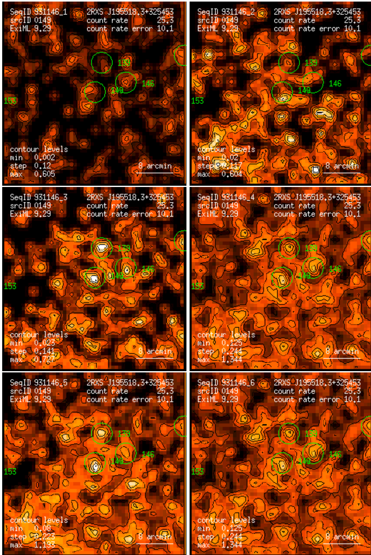
Figure 149: RASS 931146: detection 0149: band rate images, Gaussian filter: (1) PSPC channels 11 – 41, (2) 52 – 90, (3) 91 – 201, (4) 11 – 235, (5) 52 – 201, (6) 11 – 201. Broad band rates in counts/ks. Band rate contour levels in counts/ks/arcmin 2 .
