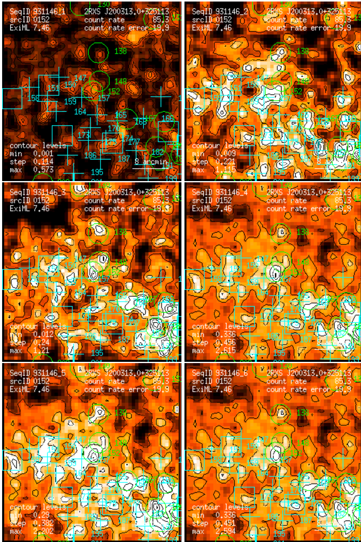
Figure 152: RASS 931146: detection 0152: band rate images, Gaussian filter: (1) PSPC channels 11 – 41, (2) 52 – 90, (3) 91 – 201, (4) 11 – 235, (5) 52 – 201, (6) 11 – 201. Broad band rates in counts/ks. Band rate contour levels in counts/ks/arcmin 2 .
