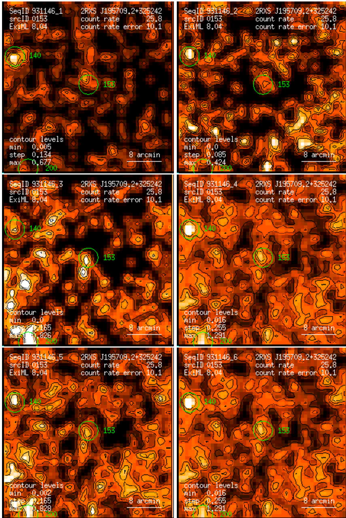
Figure 153: RASS 931146: detection 0153: band rate images, Gaussian filter: (1) PSPC channels 11 – 41, (2) 52 – 90, (3) 91 – 201, (4) 11 – 235, (5) 52 – 201, (6) 11 – 201. Broad band rates in counts/ks. Band rate contour levels in counts/ks/arcmin 2 .
