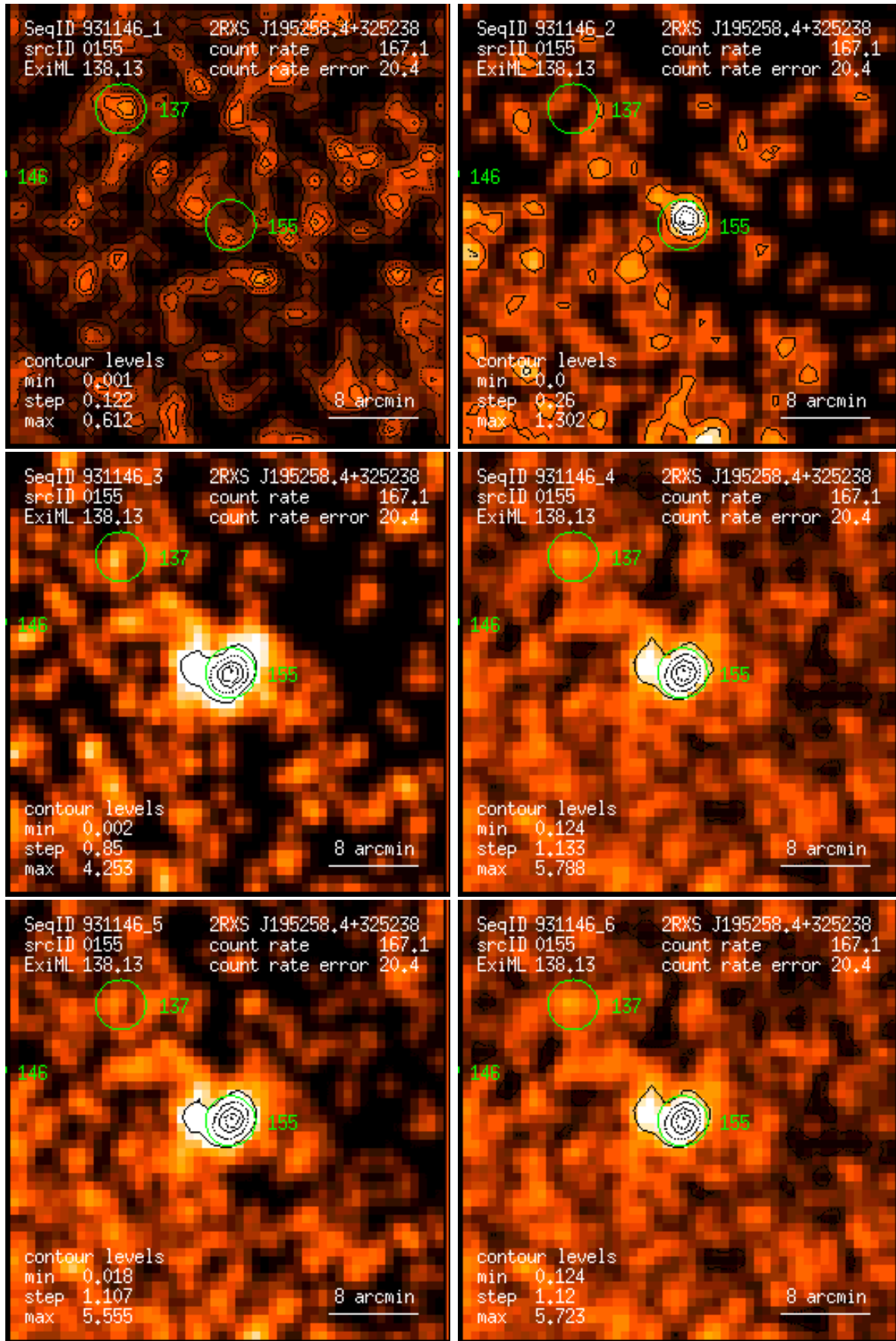
Figure 155: RASS 931146: detection 0155: band rate images, Gaussian filter: (1) PSPC channels 11 – 41, (2) 52 – 90, (3) 91 – 201, (4) 11 – 235, (5) 52 – 201, (6) 11 – 201. Broad band rates in counts/ks. Band rate contour levels in counts/ks/arcmin 2 .
