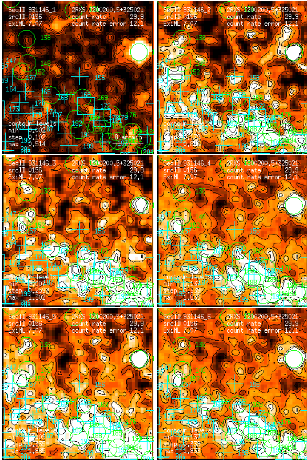
Figure 156: RASS 931146: detection 0156: band rate images, Gaussian filter: (1) PSPC channels 11 – 41, (2) 52 – 90, (3) 91 – 201, (4) 11 – 235, (5) 52 – 201, (6) 11 – 201. Broad band rates in counts/ks. Band rate contour levels in counts/ks/arcmin 2 .
