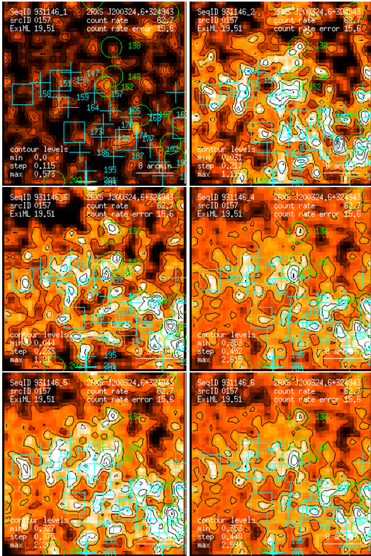
Figure 157: RASS 931146: detection 0157: band rate images, Gaussian filter: (1) PSPC channels 11 – 41, (2) 52 – 90, (3) 91 – 201, (4) 11 – 235, (5) 52 – 201, (6) 11 – 201. Broad band rates in counts/ks. Band rate contour levels in counts/ks/arcmin 2 .
