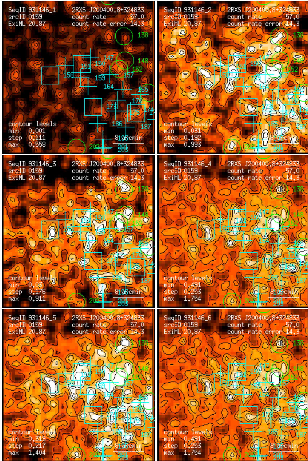
Figure 159: RASS 931146: detection 0159: band rate images, Gaussian filter: (1) PSPC channels 11 – 41, (2) 52 – 90, (3) 91 – 201, (4) 11 – 235, (5) 52 – 201, (6) 11 – 201. Broad band rates in counts/ks. Band rate contour levels in counts/ks/arcmin 2 .
