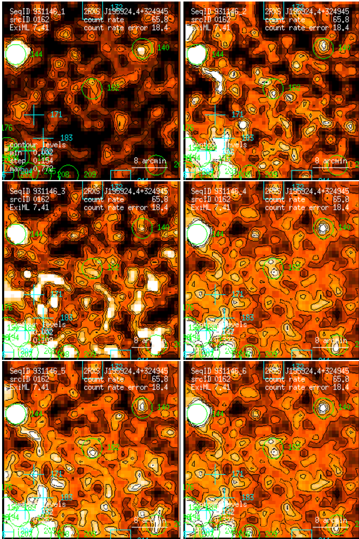
Figure 162: RASS 931146: detection 0162: band rate images, Gaussian filter: (1) PSPC channels 11 – 41, (2) 52 – 90, (3) 91 – 201, (4) 11 – 235, (5) 52 – 201, (6) 11 – 201. Broad band rates in counts/ks. Band rate contour levels in counts/ks/arcmin 2 .
