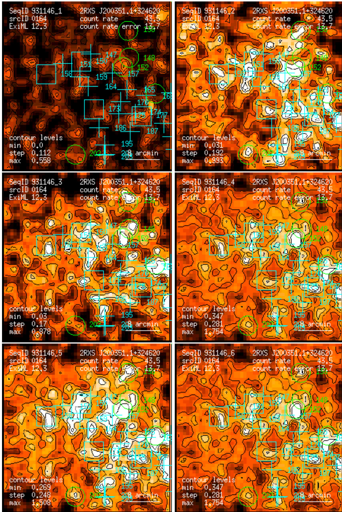
Figure 164: RASS 931146: detection 0164: band rate images, Gaussian filter: (1) PSPC channels 11 – 41, (2) 52 – 90, (3) 91 – 201, (4) 11 – 235, (5) 52 – 201, (6) 11 – 201. Broad band rates in counts/ks. Band rate contour levels in counts/ks/arcmin 2 .
