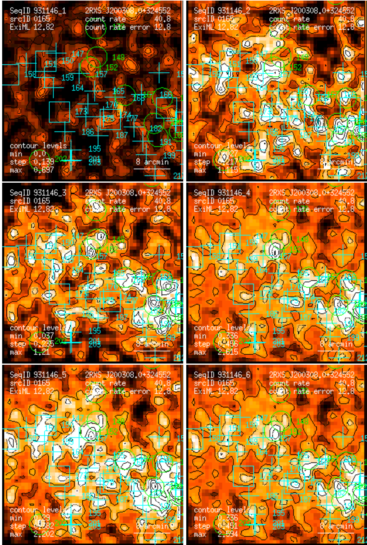
Figure 165: RASS 931146: detection 0165: band rate images, Gaussian filter: (1) PSPC channels 11 – 41, (2) 52 – 90, (3) 91 – 201, (4) 11 – 235, (5) 52 – 201, (6) 11 – 201. Broad band rates in counts/ks. Band rate contour levels in counts/ks/arcmin 2 .
