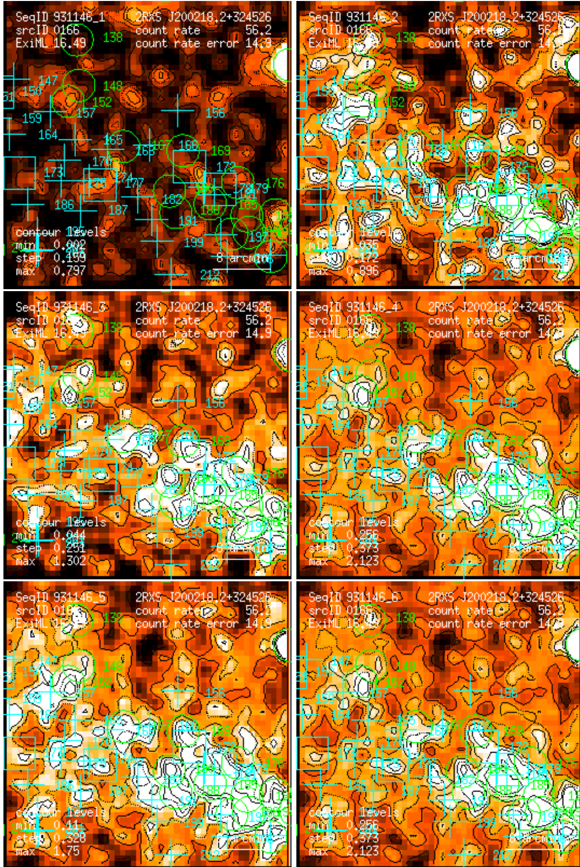
Figure 166: RASS 931146: detection 0166: band rate images, Gaussian filter: (1) PSPC channels 11 – 41, (2) 52 – 90, (3) 91 – 201, (4) 11 – 235, (5) 52 – 201, (6) 11 – 201. Broad band rates in counts/ks. Band rate contour levels in counts/ks/arcmin 2 .
