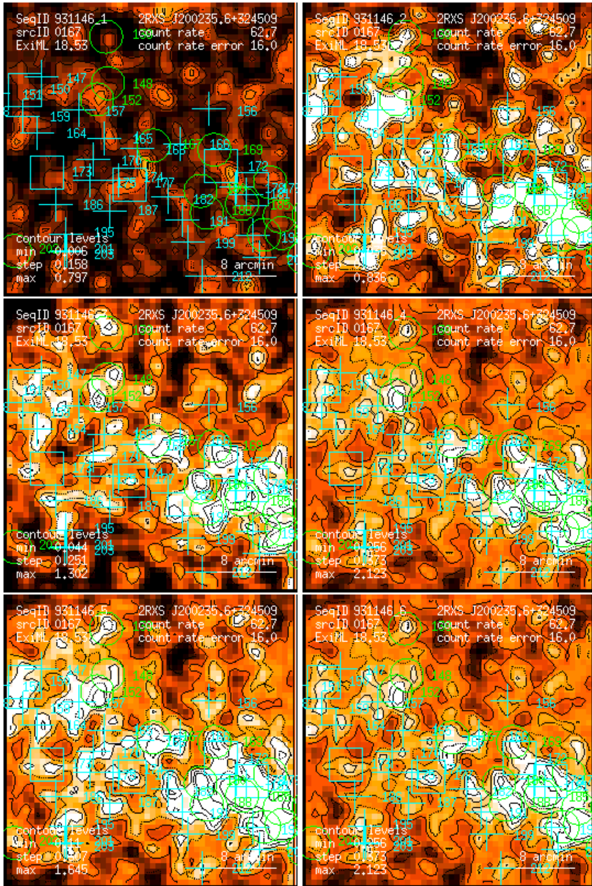
Figure 167: RASS 931146: detection 0167: band rate images, Gaussian filter: (1) PSPC channels 11 – 41, (2) 52 – 90, (3) 91 – 201, (4) 11 – 235, (5) 52 – 201, (6) 11 – 201. Broad band rates in counts/ks. Band rate contour levels in counts/ks/arcmin 2 .
