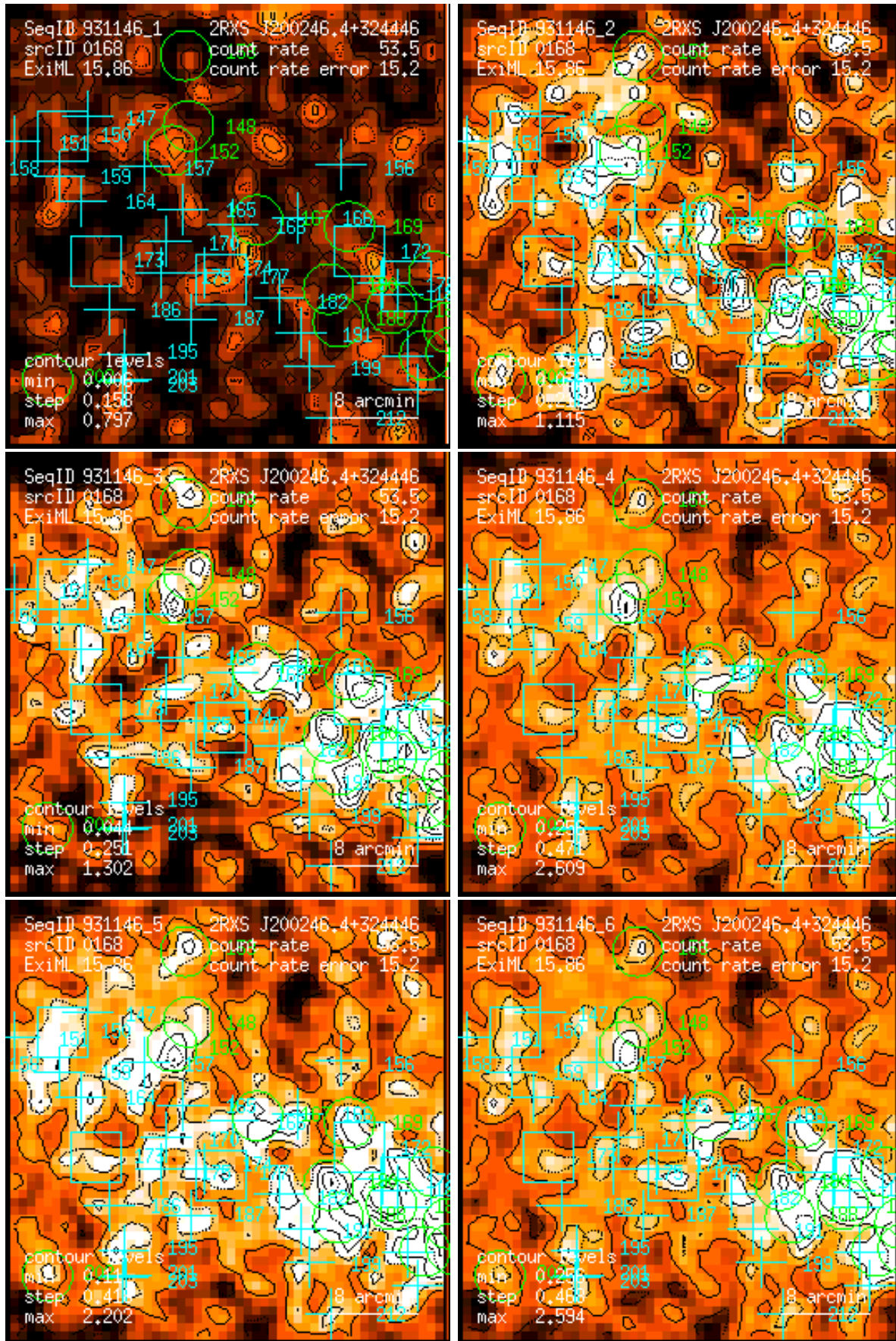
Figure 168: RASS 931146: detection 0168: band rate images, Gaussian filter: (1) PSPC channels 11 – 41, (2) 52 – 90, (3) 91 – 201, (4) 11 – 235, (5) 52 – 201, (6) 11 – 201. Broad band rates in counts/ks. Band rate contour levels in counts/ks/arcmin 2 .
